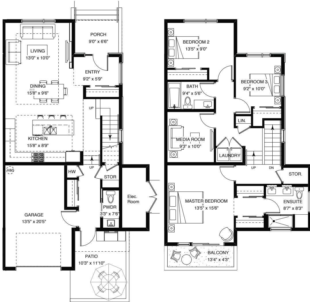
MAIN FLOOR 749 SQ FT
